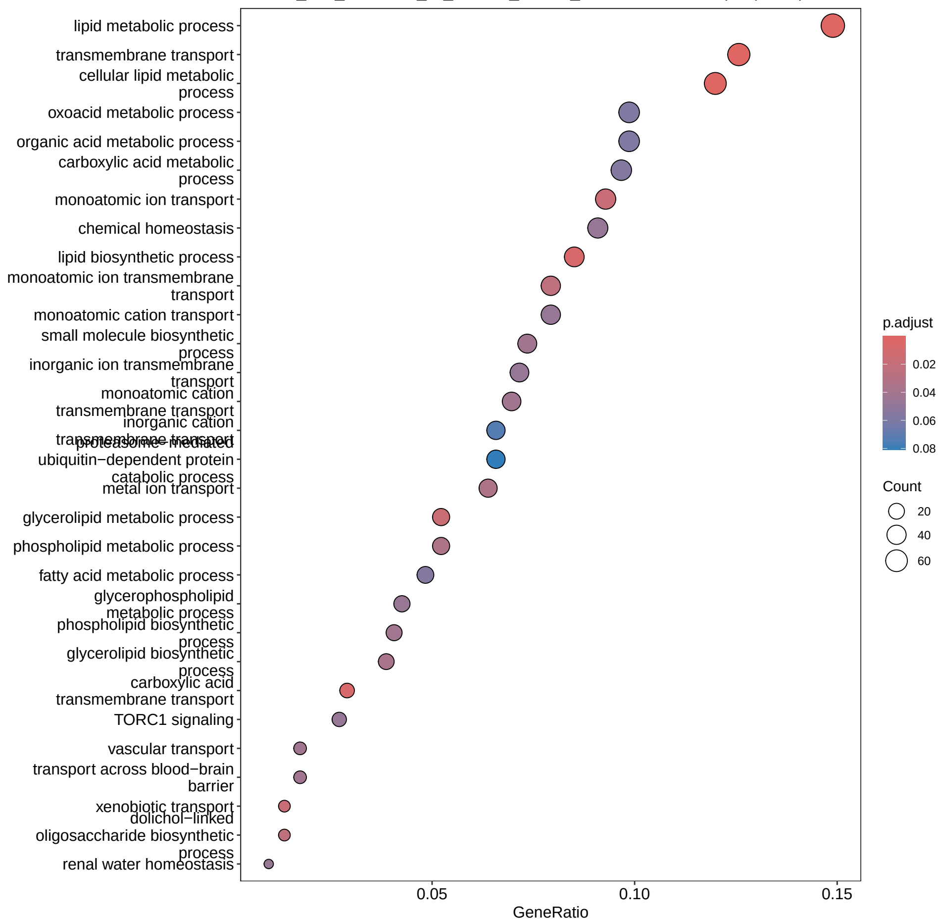
RDH12_100_atRAL5hr_vs_RDH12_control_atRAL5hr: GO BP (simplified)
